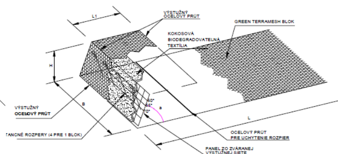
Obr.1 B Green Terramesh
